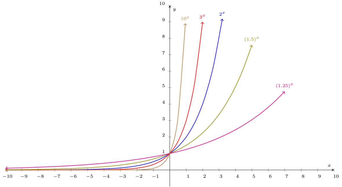
Exponential Functions
